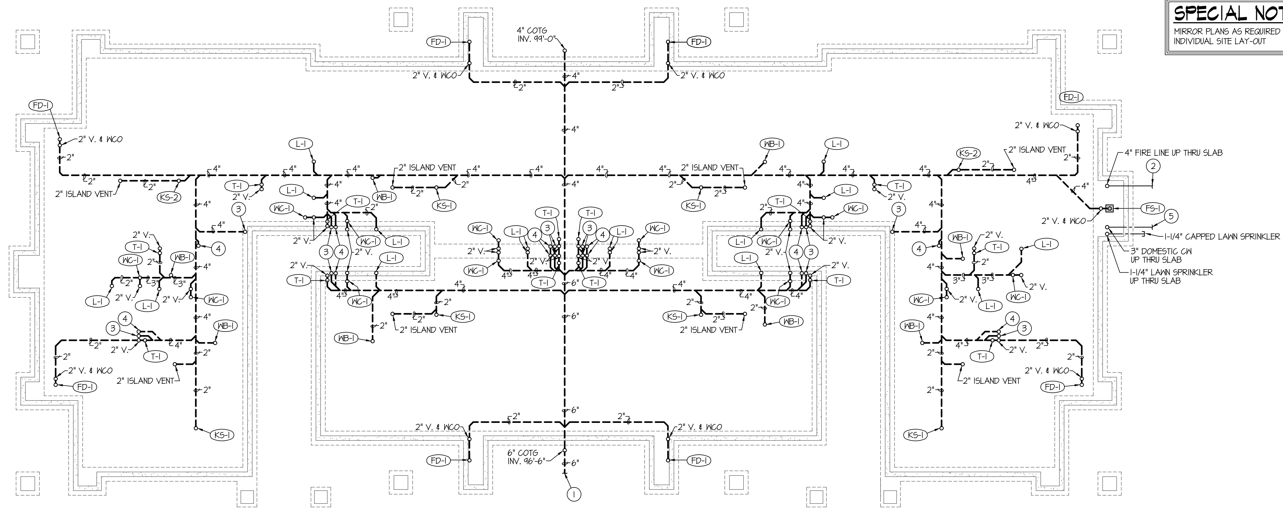
FOUNDATION PLUMBING PLAN SCALE: 1/8" = 1'-0"
